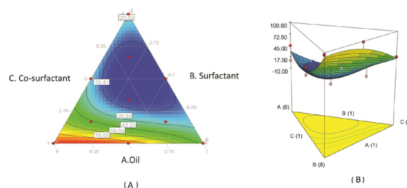
Figure 1: (A) Counter plot response of transmittance, (B) 3D Surface response of transmittance
