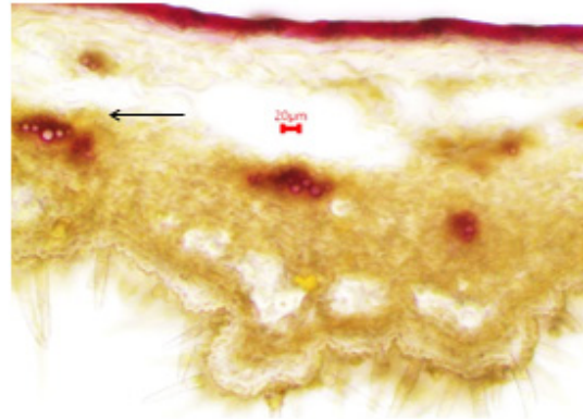
Lignin compound
