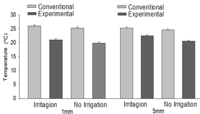
Figure 4: Average values of the block temperatures at depths of 1 mm and 5mm at 150 RPM with and without irrigation with conventional drills and experimental KOPP brand drills.
