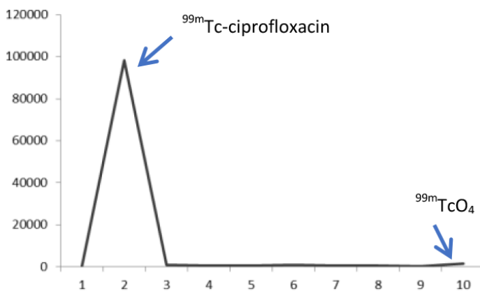
Figure 3: Chromatogram profile of ^{99m}\text{Tc} -ciprofloxacin and \text{TcO}_4^- with Whatman 1 MM/ methyl ethyl ketone.
