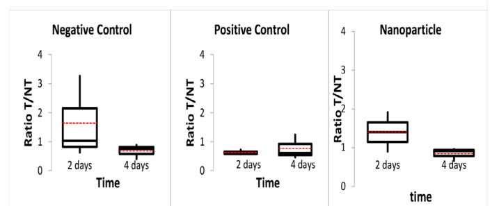
Figure 6: Boxplot diagrams of each treatment.
