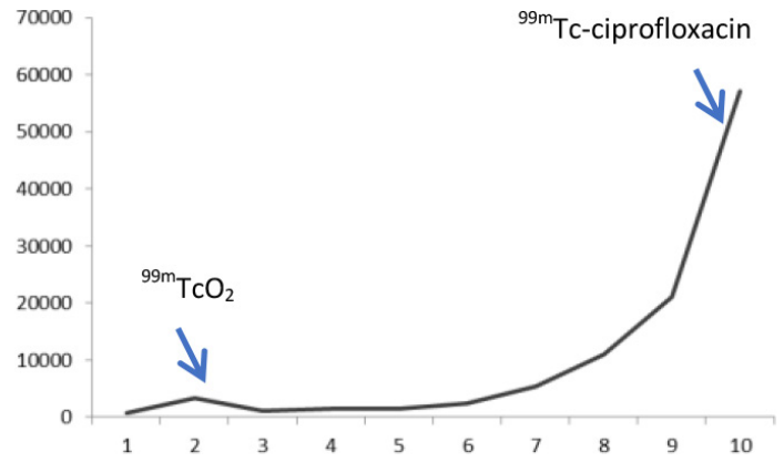
Figure 4: Chromatogram profile of ^{99m}\text{Tc} -ciprofloxacin and \text{TcO}_2 with ITLC-SG/ Et-OH/ \text{H}_2\text{O}/\text{NH}_3 (2:5:1).
